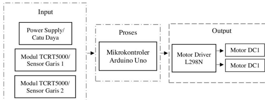
Gambar 2 Blok Diagram Sistem Line Follower
