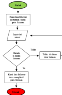
Gambar 3 Flowchart Sistem
