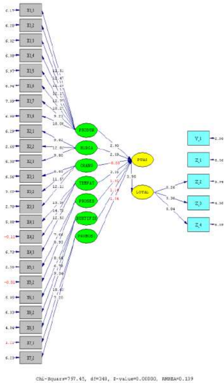
Gambar 2. Hasil Analisis Model SEM Loading Factor
