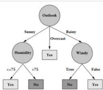
Fig. 2. Decision tree induced by C4.5.
